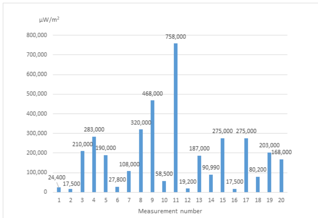
Figure 4: Results of 20 measurements in \mu\text{W}/\text{m}^2 , each during 1 minute, for peak radiation from 5G in the living room 30 cm from the window
